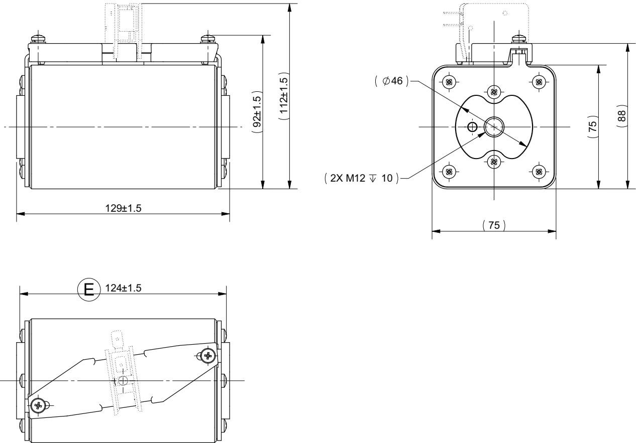
Dimensions (mm) - Size 3, 170M2010 to 170M2016, Flush end
