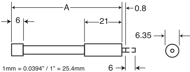
Dimensions (mm)
