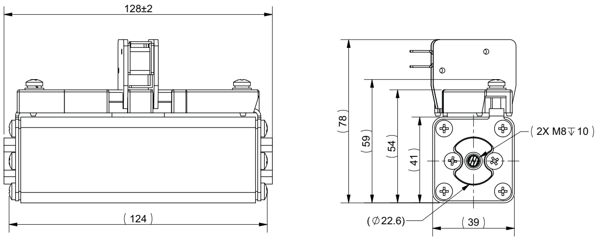
Dimensions (mm) - Size 1*, 170M2000 to 170M2005, Flush end
